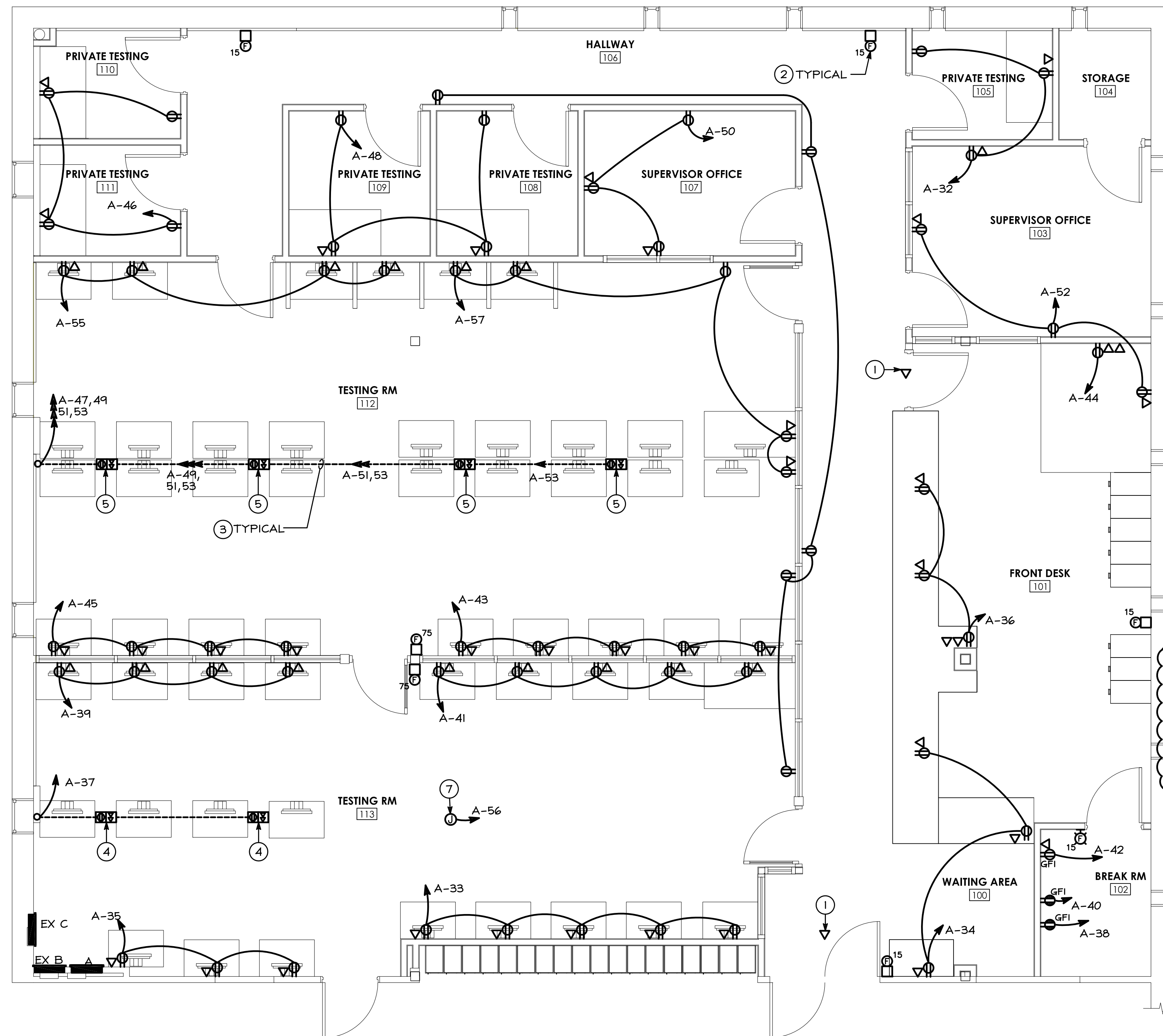
FLOOR PLAN - POWER SCALE: 1/4"=1'-0"
